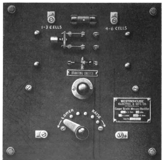
Type E Mercury Rectifier for Charging Ignition Batteries.
